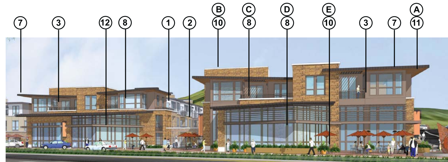
Ⓕ EXTERIOR LIGHT VISA LIGHTING: WALL SCONCE, 23 FIXTURES 150 W MAX, 10" x 33" x 13"
